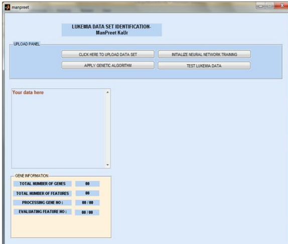
Fig 3.2: GUI interface
